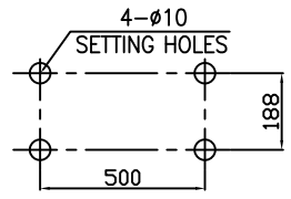
SETTING DIMENSION
